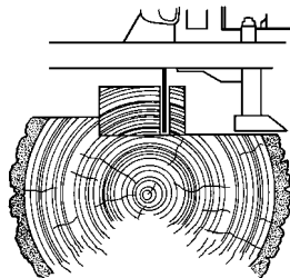
Use pre-cut log to hold cants for re-sawing
